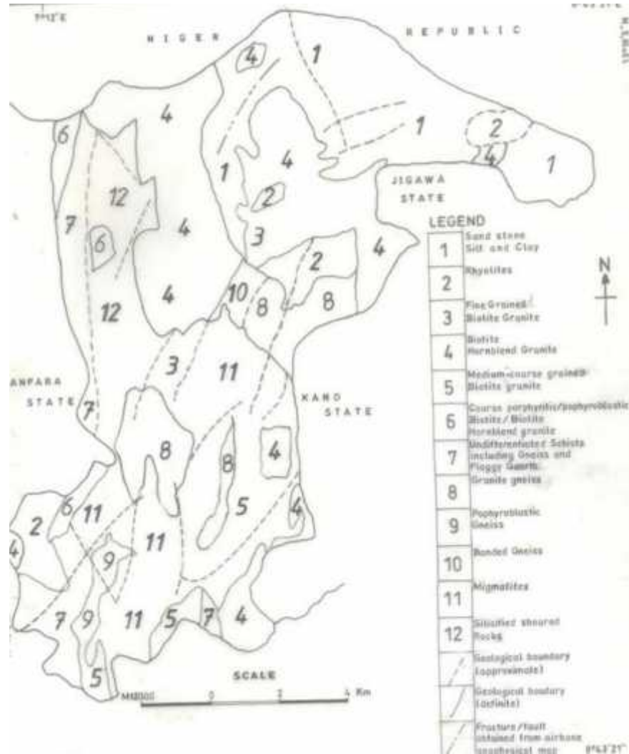
Figure 3: Geological map of Katsina State.
